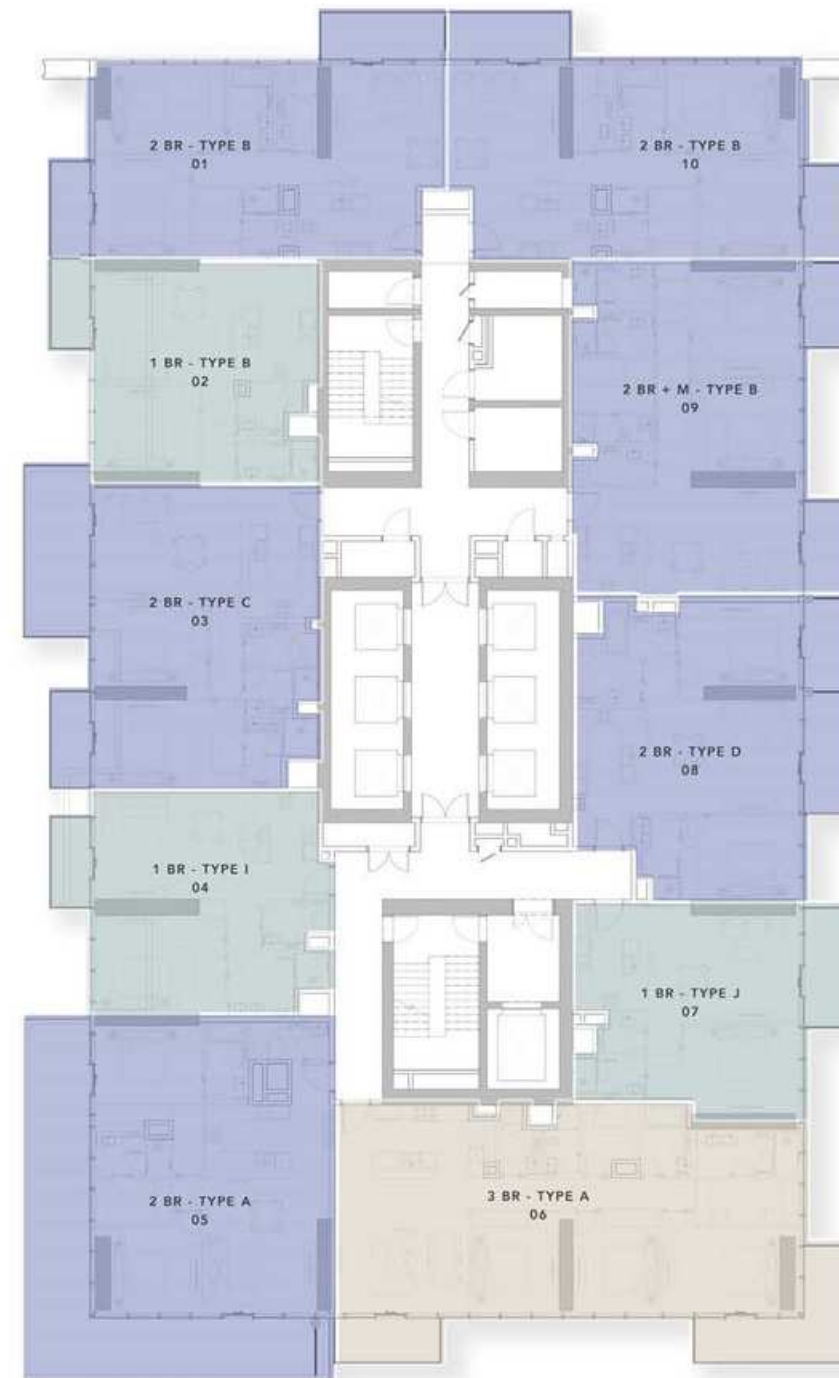
25TH FLOOR PLAN
